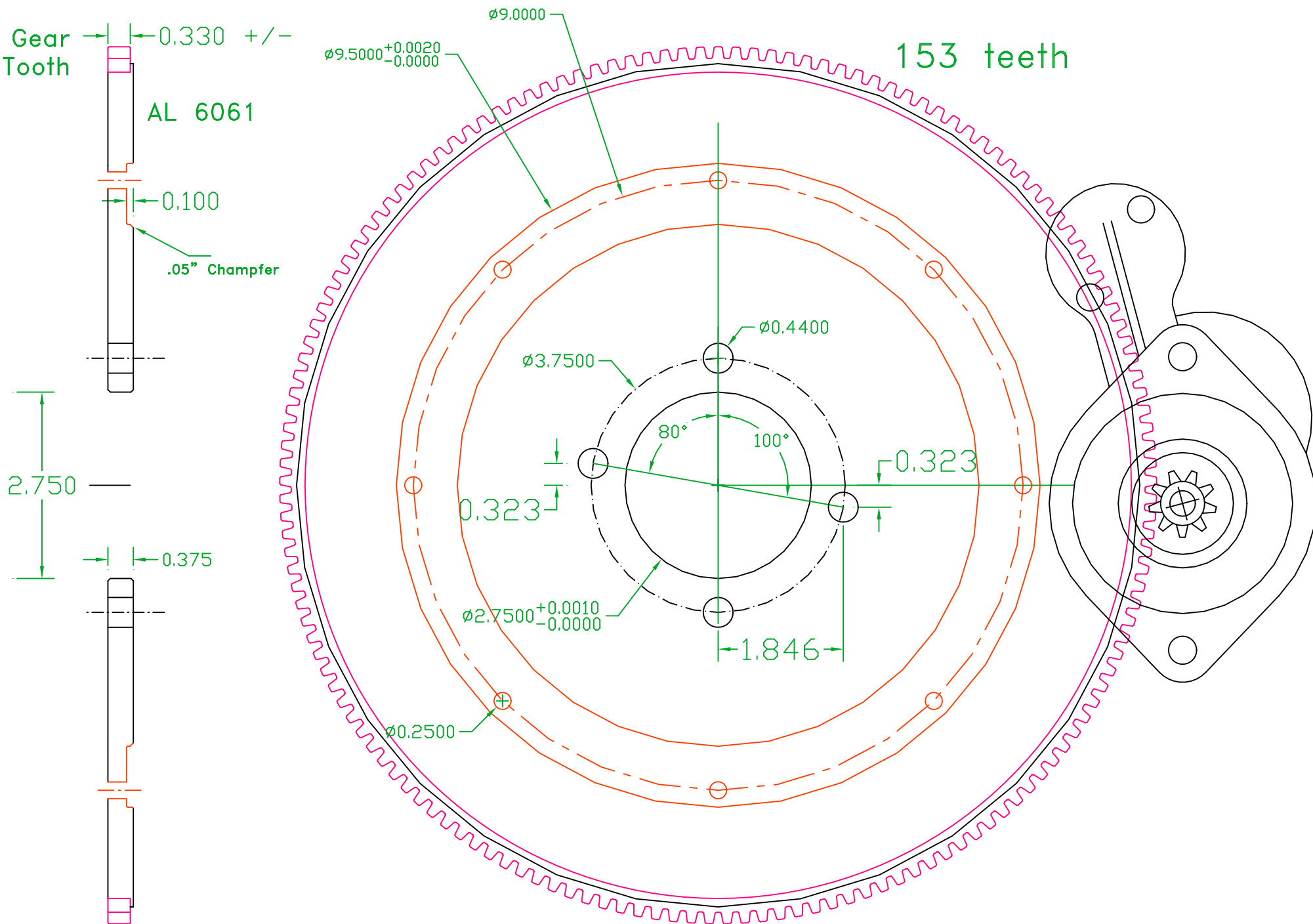
Bolt Pattern for Stuska Dyno Flange
